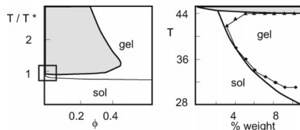
Figure 5. On the left panel, a theoretical phase diagram for parameter values of N = 3000 , s = 17 , E = -17 , and g = -1.5 . Marked by a rectangle is the region of convergence of gel, sol, and phase separated regions. On the right, a comparison of this region with experimentally determined boundaries for p-(NIPAAm-co-acrylic acid) obtained by Han and Bae. 14 The units in the left panel correspond to the dimensionless model variables. Temperatures in ^{\circ}\text{C} in the right panel.
